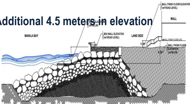
MALL OF ASIA COMPLEX SEAWALL DETAIL SCALE: 1/11
